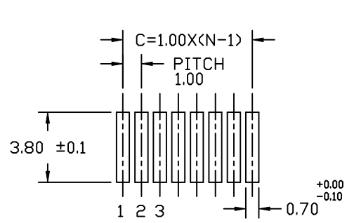
RECOMMENDED PCB LAYOUT FOR SURFACE MOUNT
